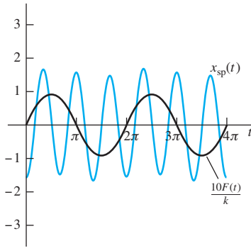
FIGURE 8.4.7. The imposed force and the resulting steady periodic motion in Example 4.
