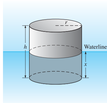
FIGURE 2.4.12. The buoy of Problem 10.
