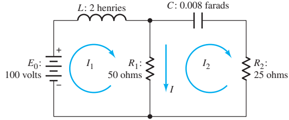
FIGURE 5.1.4. The electrical network of Example 3.
