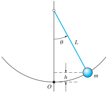
FIGURE 2.4.3. The simple pendulum.
