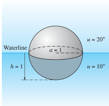
FIGURE 9.5.10. A floating spherical buoy with specific gravity \delta = 0.5 .
