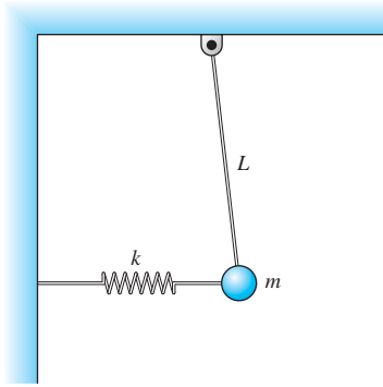
FIGURE 2.6.10. The pendulum-and-spring system of Problem 21.
