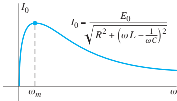
FIGURE 2.7.6. The effect of frequency on I_0 .
