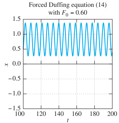
FIGURE 7.6.13(b). Period 2\pi response with F_0 = 0.60 : solution x(t) .
