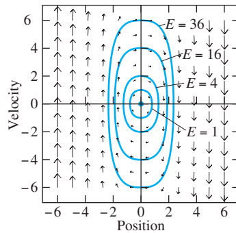
FIGURE 7.5.2. Position-velocity phase plane portrait for the hard mass-and-spring system with m = k = 2 and \beta = -4 < 0 .
