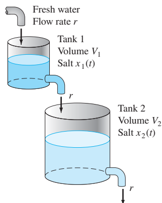
FIGURE 5.4.7. The two brine tanks of Problems 27 and 28.
