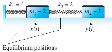
FIGURE 5.2.2. The mass–and–spring system of Example 3.
