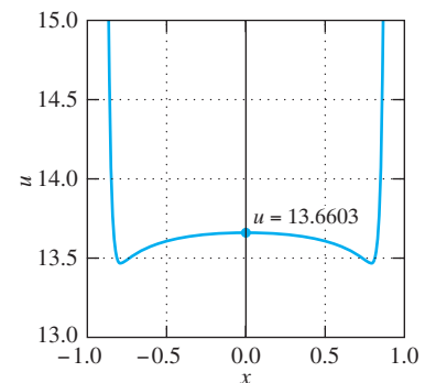
FIGURE 9.5.14. The temperature u(x) in the waterline cross section of the buoy with h = 0.5 .
