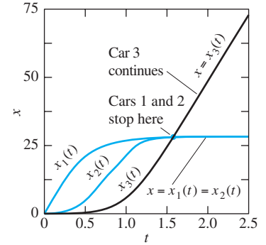
FIGURE 5.5.8. Position functions of the three railway cars of Example 2.
