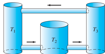
FIGURE 5.1.13. The fermentation tanks of Problem 26.
