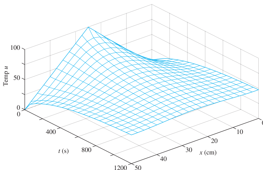
FIGURE 8.5.6. The graph of the temperature function u(x, t) in Example 3.
