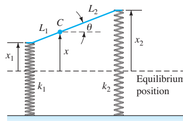
FIGURE 5.5.14. Model of the two-axle automobile.
