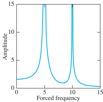
FIGURE 5.5.10. Frequency–amplitude plot for Example 3.
