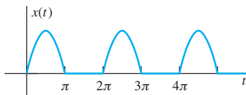
FIGURE 4.6.5. The half-wave rectification of \sin t .
