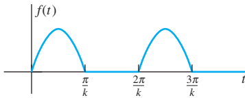
FIGURE 4.5.16. The half-wave rectification of \sin kt .
