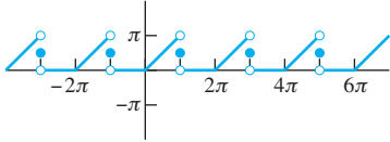
FIGURE 8.1.4. The periodic function of Example 2.
