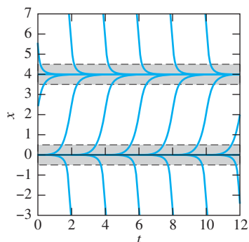
FIGURE 7.1.4. Solution curves, funnel, and spout for dx/dt = 4x - x^2 .
