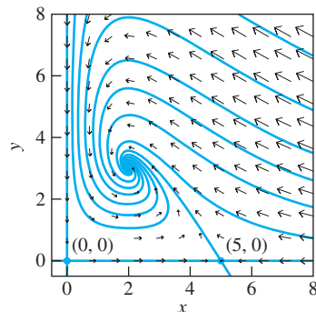
FIGURE 7.4.14. Direction field and phase portrait for the predator–prey system of Problems 11 through 13.
