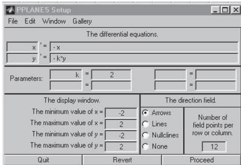
FIGURE 7.2.20. MATLAB pplane menu entries to plot a direction field and phase portrait for the system x' = -x , y' = -2y (as shown in Fig. 7.2.6).
