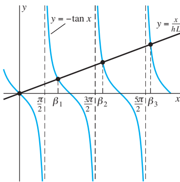
FIGURE 9.1.1. The solution of Eq. (17) by geometric methods.
