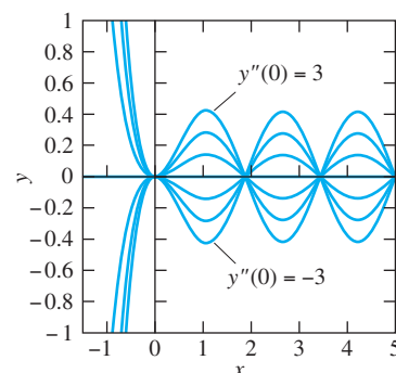
FIGURE 2.2.4. Solutions of y^{(3)} + 3y'' + 4y' + 12y = 0 with y(0) = y'(0) = 0 but with different values for y''(0) .
