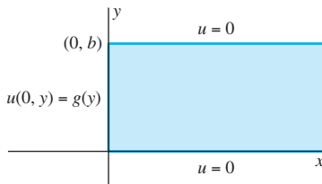
FIGURE 8.7.5. The “semi-infinite” strip of Example 2.
