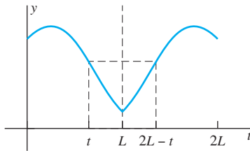
FIGURE 8.3.7. Construction of F from f in Problem 21.
