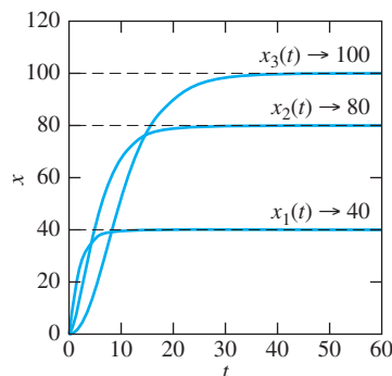
FIGURE 5.8.2. The salt amount solution curves defined in (8).
