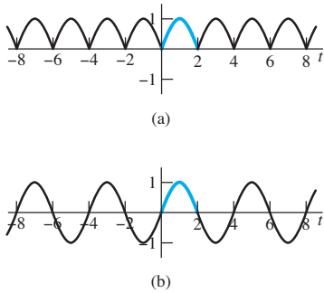
FIGURE 8.3.3. (a) The period 4 even extension of f(t) = 2t - t^2 for 0 < t < 2 . (b) Graph of the period 4 odd extension of f(t) = 2t - t^2 for 0 < t < 2 .
