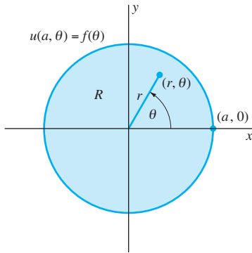
FIGURE 8.7.7. The Dirichlet problem for a circular disk.
