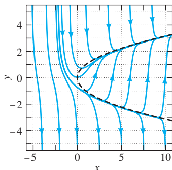
FIGURE 3.6.7. Solution curves of \frac{dy}{dx} = x - y^2 .
