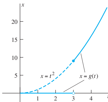
FIGURE 4.5.4. The graph of the function g(t) of Example 2.
