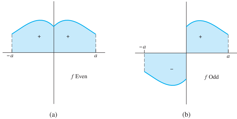
FIGURE 8.3.2. Area under the graph of (a) an even function and (b) an odd.
