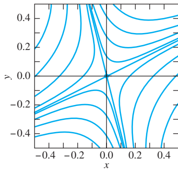
FIGURE 7.3.13. Trajectories of the linearized system of Example 7.
