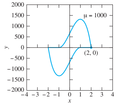
FIGURE 7.5.20. The phase plane trajectory of the periodic solution of van der Pol's equation with \mu = 1000 .
