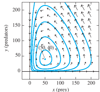
FIGURE 7.4.2. The predator–prey phase portrait of Example 2.
