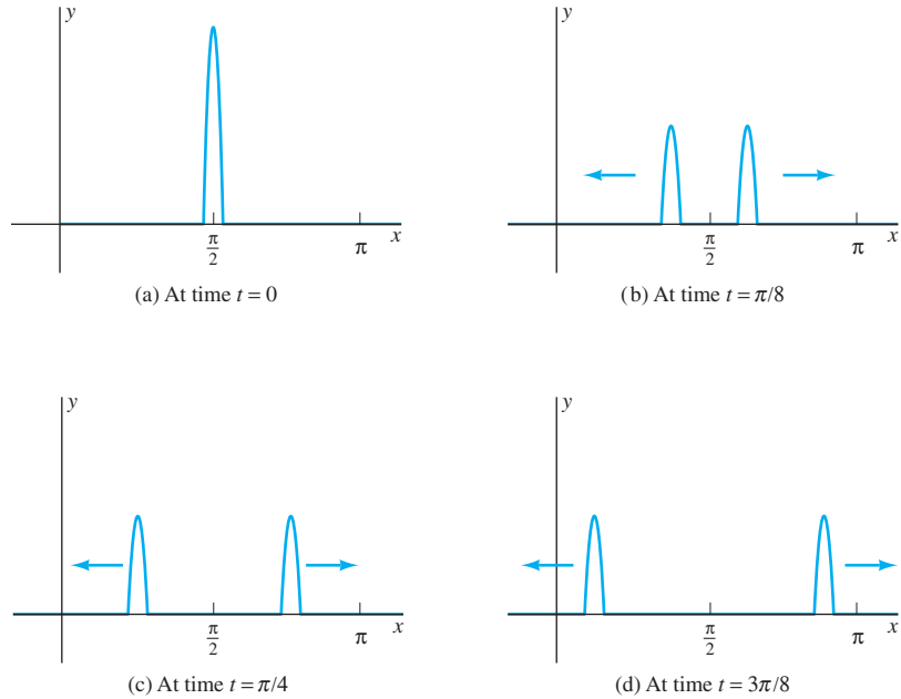
FIGURE 8.6.3. The pulse F(x) produces two waves—one moving to the left, one to the right.
