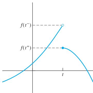
FIGURE 8.2.2. A finite jump discontinuity.
