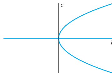
FIGURE 7.1.13. Bifurcation diagram for dx/dt = kx - x^3 .
