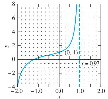
FIGURE 6.1.12. Solution of dy/dx = x^2 + y^2 , y(0) = 1 .
