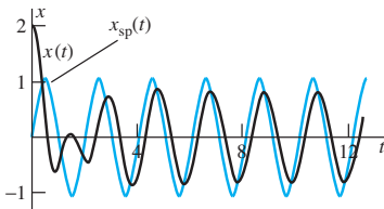
FIGURE 8.4.8. The steady periodic solution x_{\text{sp}}(t) and the damped solution x(t) .
