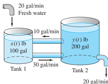
FIGURE 5.1.3. The two brine tanks of Example 2.
