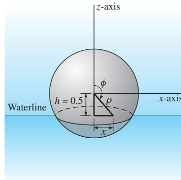
FIGURE 9.5.13. The waterline cross section with z = -0.5 , -\frac{\sqrt{3}}{2} \leq x \leq \frac{\sqrt{3}}{2} .
