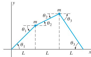
FIGURE 5.1.12. The mechanical system of Problem 25.
