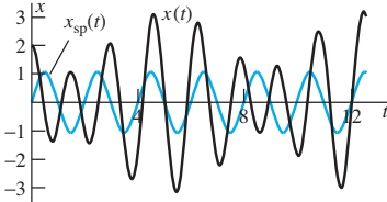
FIGURE 8.4.4. The steady periodic solution x_{\text{sp}}(t) and the nonperiodic solution x(t) .
