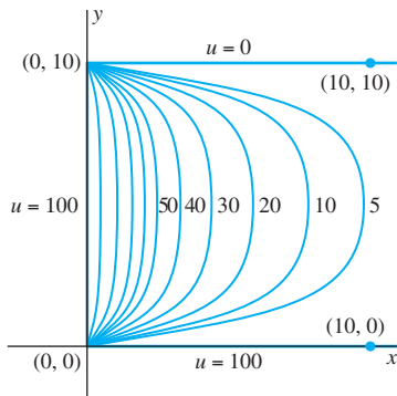
FIGURE 8.7.6. Typical level curves of the function u(x, y) of Example 2.
