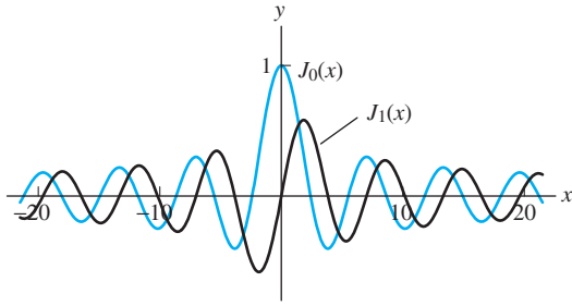
FIGURE 3.5.2. The graphs of the Bessel functions J_0(x) and J_1(x) .
