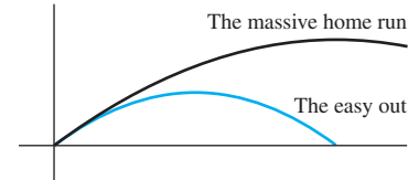
FIGURE 6.4.7. An “easy out” or a home run?
