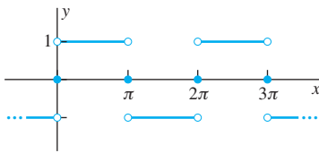
FIGURE 8.1.1. A square-wave function.
