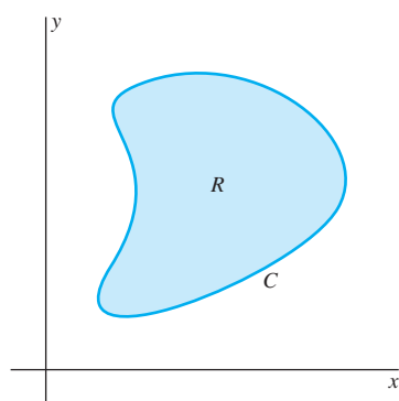
FIGURE 8.7.1. A plane region R and its bounding curve C .
