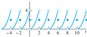
FIGURE 8.2.3. The period 2 function of Example 2.
