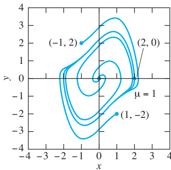
FIGURE 7.5.18. The phase plane trajectory of a periodic solution of van der Pol's equation with \mu = 1 , as well as some trajectories spiraling in and out.
