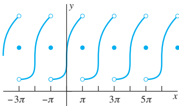
FIGURE 8.1.2 Extending a function to produce a periodic function.
