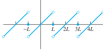
FIGURE 8.3.5. The odd period 2L extension of f .
