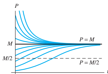
FIGURE 1.7.3. Typical solution curves for the logistic equation P' = kP(M - P) . Each solution curve that starts below the line P = M/2 has an inflection point on this line. (See Problem 34.)
