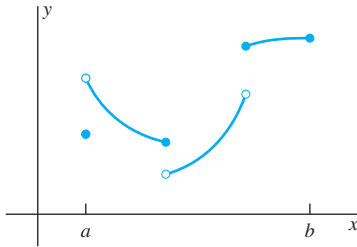
FIGURE 4.1.3. The graph of a piecewise continuous function; the solid dots indicate values of the function at discontinuities.
