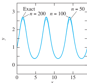
FIGURE 6.2.9. Approximating the exact solution y = e^{\sin x} using the improved Euler method with n = 50 , n = 100 , and n = 200 subintervals.
