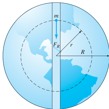
FIGURE 2.4.13. A mass m falling down a hole through the center of the earth (Problem 12).
