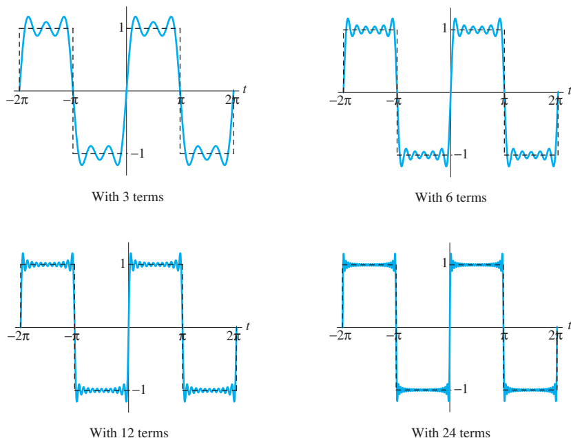
FIGURE 8.1.3. Graphs of partial sums of the Fourier series of the square-wave function (Example 1) with N = 3, 6, 12 , and 24 terms.
