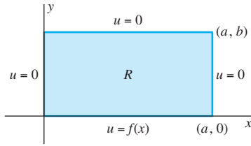
FIGURE 8.7.3. The boundary value problem of Example 1.
