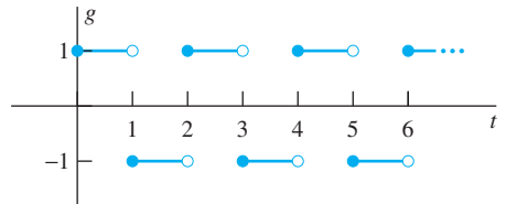
FIGURE 4.1.11. The graph of the function of Problem 41.
