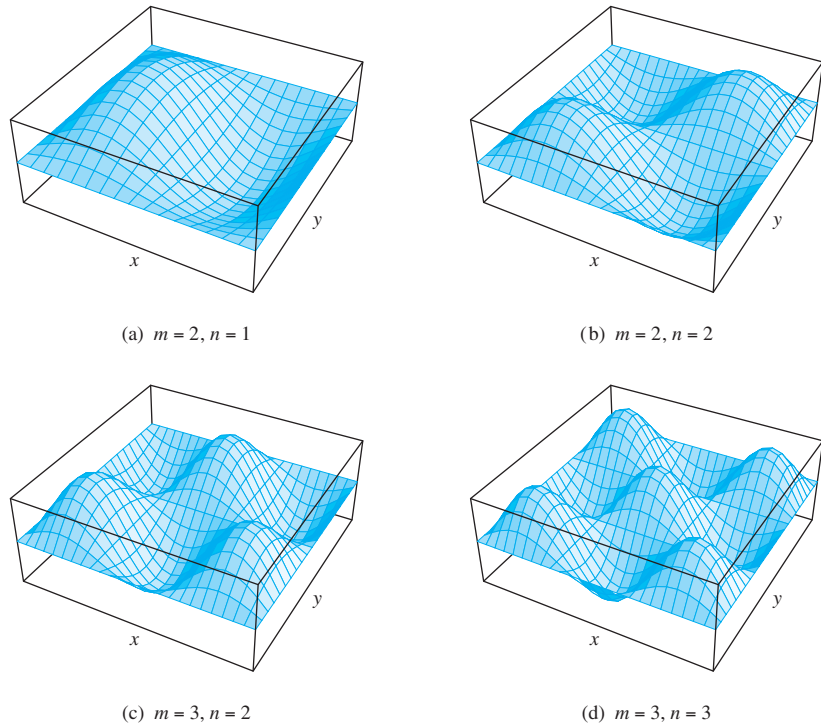
FIGURE 9.5.1. Surfaces of the form u = \sin \frac{m\pi x}{a} \sin \frac{n\pi y}{b} .
