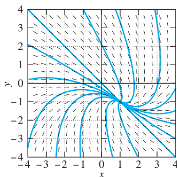
FIGURE 7.2.13. Spiral point (1, -1) .
