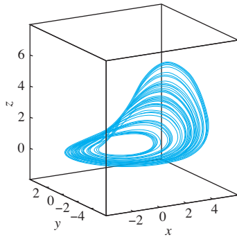
FIGURE 7.6.20. The Rössler band illustrated with a trajectory plotted with x(0) = 2 , y(0) = 0 , z(0) = 3 , and 0 \leq t \leq 400 .
