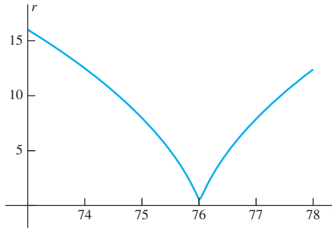
FIGURE 6.4.17. A closer look at Halley's perihelion passage after about 76 years.
