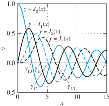
FIGURE 9.5.5. The graphs and initial zeros of the first several Bessel functions.
