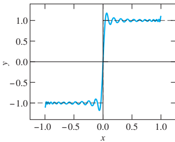
FIGURE 9.5.9. The graph of the 25-term partial sum of the rectangular wave series in Eq. (66).
