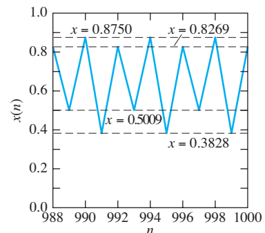
FIGURE 7.6.5. The graph of x(n) = x_n , showing the period 4 cycle of iterates obtained with r = 3.5 .
