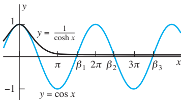
FIGURE 9.3.2. Solutions of \cosh x \cos x = 1 .
