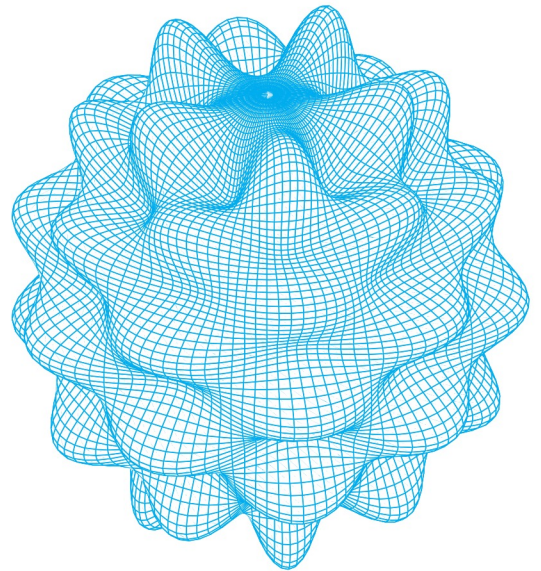
FIGURE 9.5.16. With m = 5 and n = 13 .
