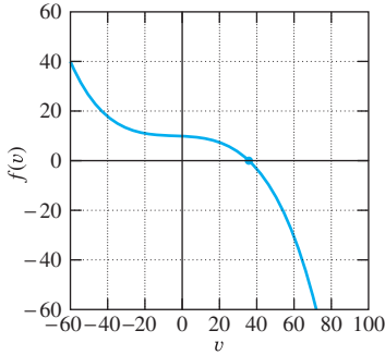
FIGURE 6.3.7. Graph of f(v) = 9.8 - (0.00016)(100v + 10v^2 + v^3) .
