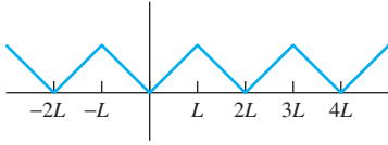
FIGURE 8.3.4. The even period 2L extension of f .
