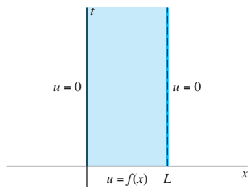
FIGURE 8.5.2. A geometric interpretation of the boundary value problem in Eqs. (12a)–(12c).
