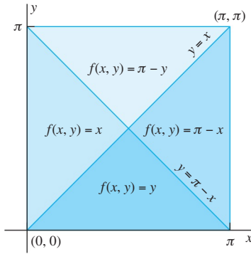
FIGURE 9.5.2. Piecewise definition of the tent function.
