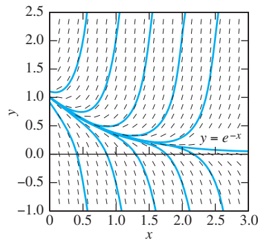
FIGURE 6.3.10. Direction field and solution curves for dy/dx = 5y - 6e^{-x} .
