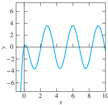
FIGURE 2.2.1. The particular solution y(x) = -3e^{-3x} + 3\cos 2x - 2\sin 2x .
