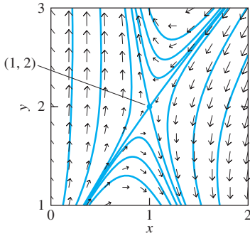
FIGURE 7.3.1. The saddle point (1, 2) for the system x' = 3x - x^2 - xy , y' = y + y^2 - 3xy of Example 1.
