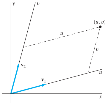
FIGURE 7.3.3. The oblique uv -coordinate system determined by the eigenvectors \mathbf{v}_1 and \mathbf{v}_2 .
