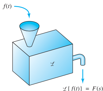
FIGURE 4.1.1. Transformation of a function: \mathcal{L} in analogy with D .
