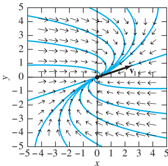
FIGURE 7.3.6. The improper nodal sink of Example 4.
