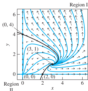
FIGURE 7.4.15. Direction field and phase portrait for the predator-prey system of Problems 14 through 17.
