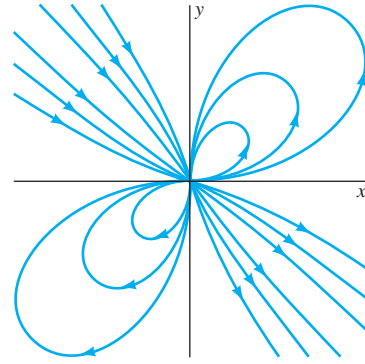
FIGURE 7.3.19. Trajectories of the system in Eq. (22).
