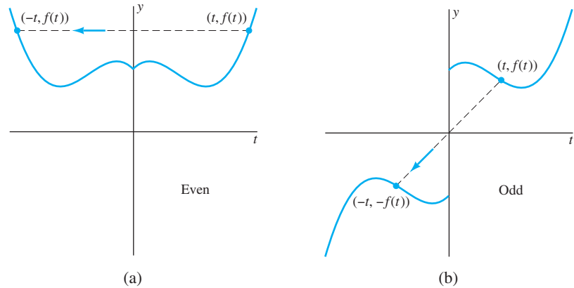
FIGURE 8.3.1. (a) An even function; (b) an odd function.
