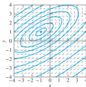
FIGURE 7.2.19. Stable center (-1, 1) .
