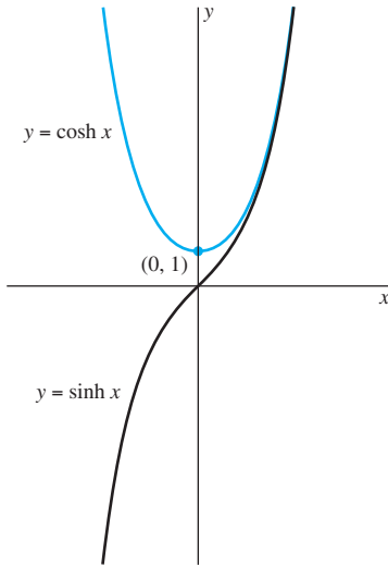
FIGURE 2.8.3. The hyperbolic sine and cosine graphs.
