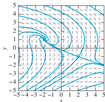
FIGURE 7.2.12. Spiral point (-2, 1) and saddle point (2, -1) .
