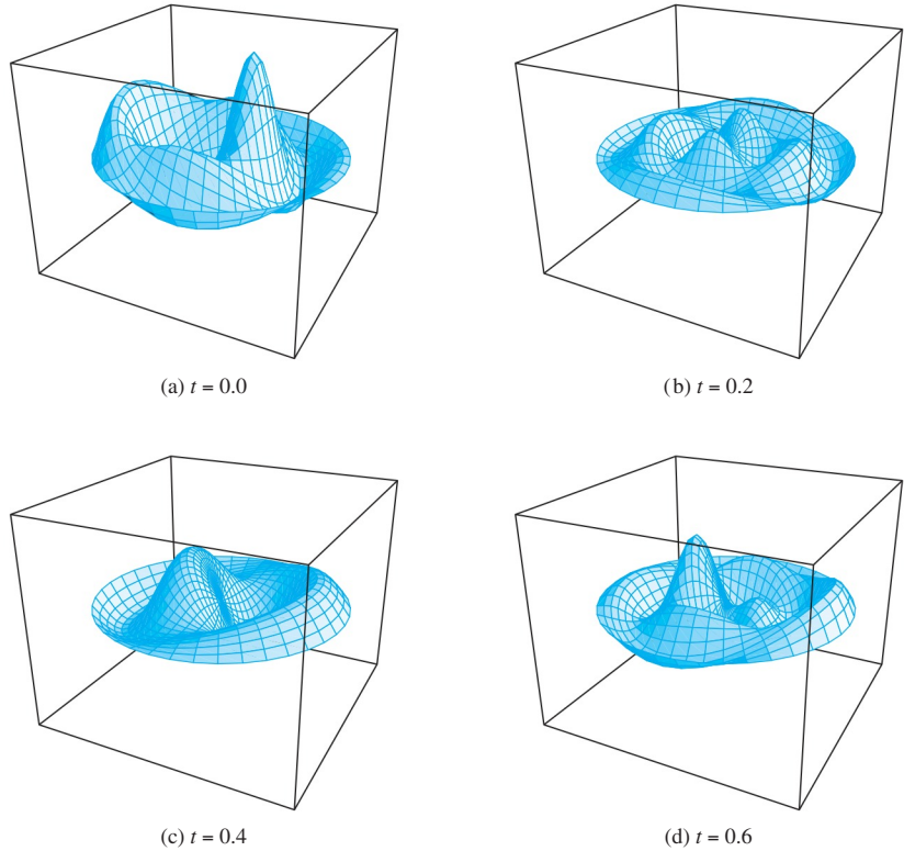
FIGURE 9.5.7. Snapshots of the circular membrane vibration defined by Eq. (54).
