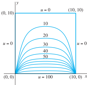
FIGURE 8.7.4. Typical level curves of the function u(x, y) in Eq. (15).
