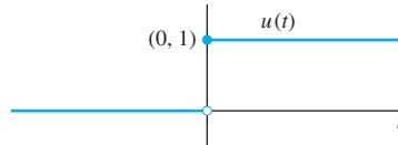
FIGURE 4.1.4. The graph of the unit step function.
