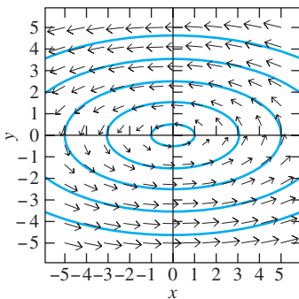
FIGURE 5.1.6. Direction field and solution curves for the system x' = -2y , y' = \frac{1}{2}x of Example 6.
