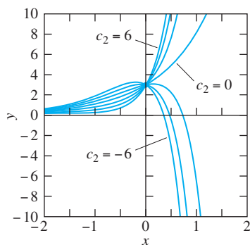
FIGURE 2.1.8. Different solutions y(x) = 3e^x + c_2 x e^x of y'' - 2y' + y = 0 with the same initial value y(0) = 3 .
