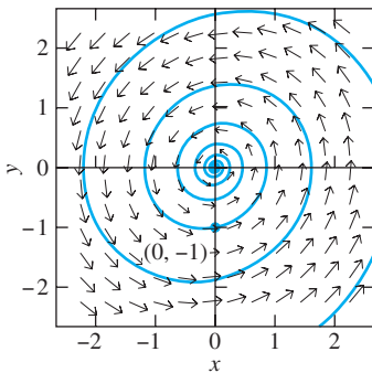
FIGURE 5.1.9. Direction field and solution curve for the system x' = -y , y' = (1.01)x - (0.2)y of Example 8.
