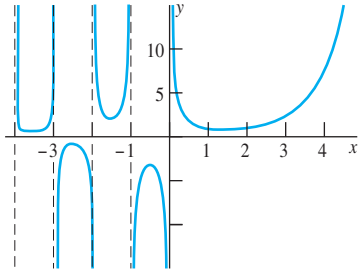
FIGURE 3.5.1. The graph of the extended gamma function.
