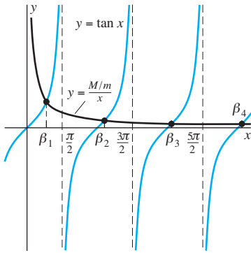
FIGURE 9.2.3. The positive roots \{\beta_n\}_1^\infty of Eq. (22).
