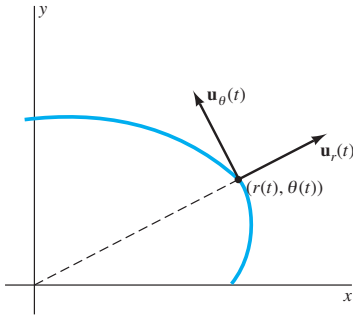
FIGURE 5.1.16. The radial and transverse unit vectors \mathbf{u}_r and \mathbf{u}_\theta .
