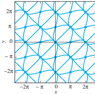
FIGURE 7.5.11. Trajectories of the system in Problem 2.
