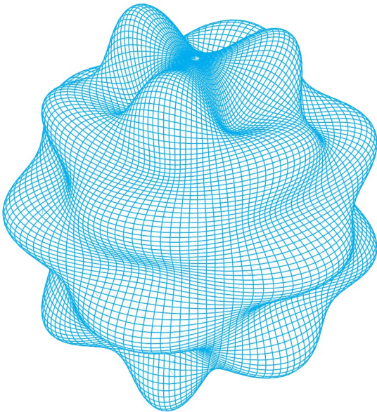
FIGURE 9.5.15. With m = 3 and n = 9 .
