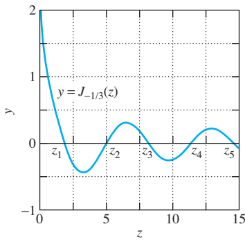
FIGURE 3.6.2. The graph of J_{-1/3}(z) .
