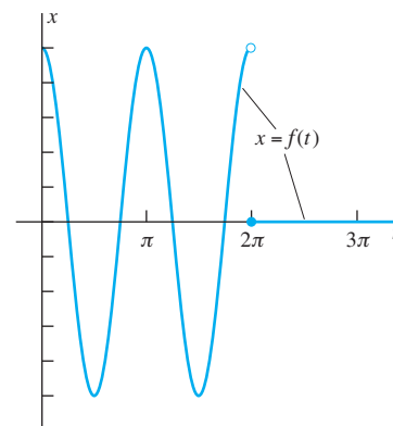
FIGURE 4.5.5. The function f(t) of Examples 3 and 4
