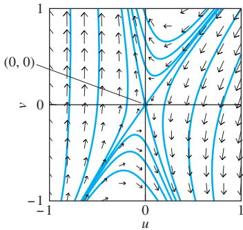
FIGURE 7.3.2. The saddle point (0, 0) for the equivalent system u' = -u - v - u^2 - uv , v' = -6u + 2v + v^2 - 3uv .
