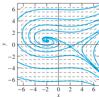
FIGURE 7.2.18. Spiral point (-2, \frac{2}{3}) and saddle point (2, -\frac{2}{3}) .
