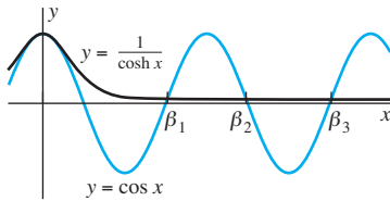
FIGURE 9.1.3. The solutions of \cosh x \cos x = 1 (the graph is not drawn to scale).
