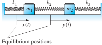
FIGURE 5.2.6. The mechanical system of Problem 38.
