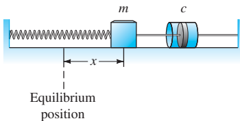
FIGURE 2.4.1. A mass-spring-dashpot system.
