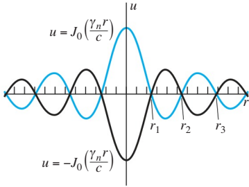
FIGURE 9.4.6. Cross section of the vibrating circular membrane.
