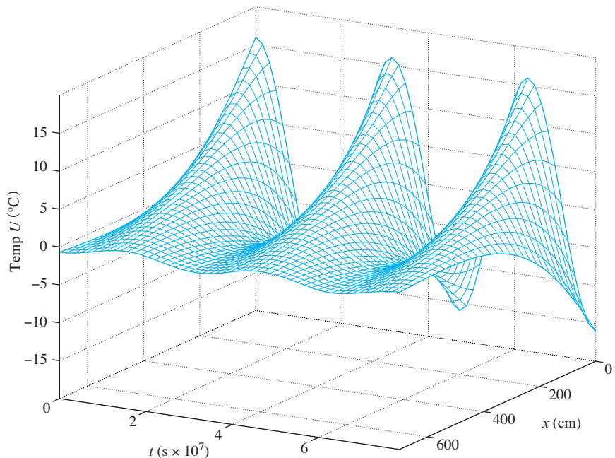
FIGURE 9.3.4. The graph of the temperature function U(x, t) in Eq. (29).
