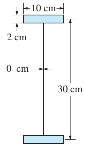
FIGURE 9.3.3. An idealized I beam.
