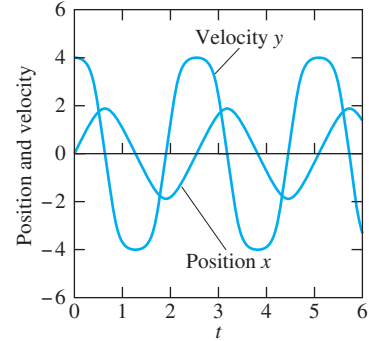
FIGURE 7.5.3. Position and velocity solution curves for the hard mass-and-spring system with m = k = 2 and \beta = -4 < 0 .
