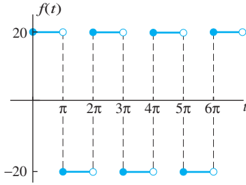
FIGURE 4.5.11. The graph of the external-force function of Example 8.
