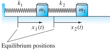
FIGURE 5.5.3. The mass-and-spring system of Example 1.
