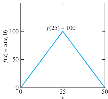
FIGURE 8.5.5. The graph of the initial temperature function u(x, 0) = f(x) in Example 3.
