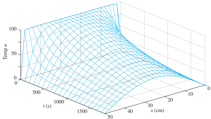
FIGURE 8.5.4. The graph of the temperature function u(x, t) in Example 2.
