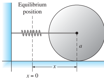
FIGURE 2.6.5. The rolling disk.
