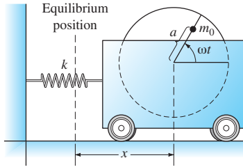
FIGURE 2.6.1. The cart-with-flywheel system.
