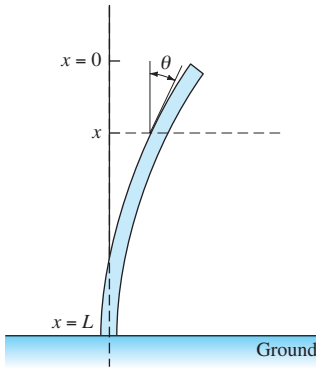
FIGURE 3.6.1. The buckling column.
