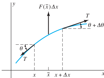
FIGURE 8.6.1. Forces on a short segment of the vibrating string.
