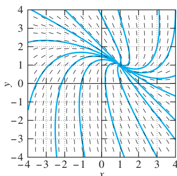
FIGURE 7.2.16. Node (1, 1) .
