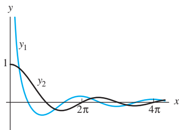
FIGURE 3.3.1. The solutions y_1(x) = \frac{\cos x}{x} and y_2(x) = \frac{\sin x}{x}
