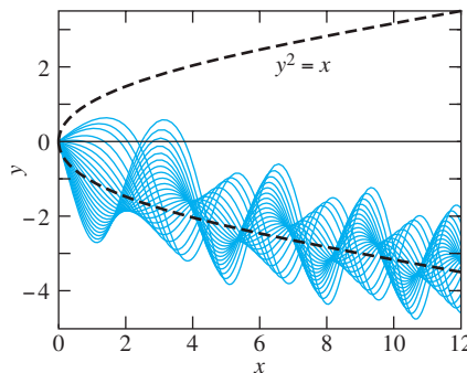
FIGURE 3.6.8. The first Painlevé transcendent y'' = y^2 - x , y(0) = 0 , y'(0) = -3.3, -3.1, \dots, 0.7 .
