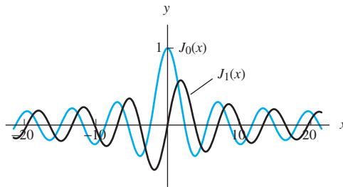
FIGURE 9.4.2. The graphs of the Bessel functions J_0(x) and J_1(x) .
