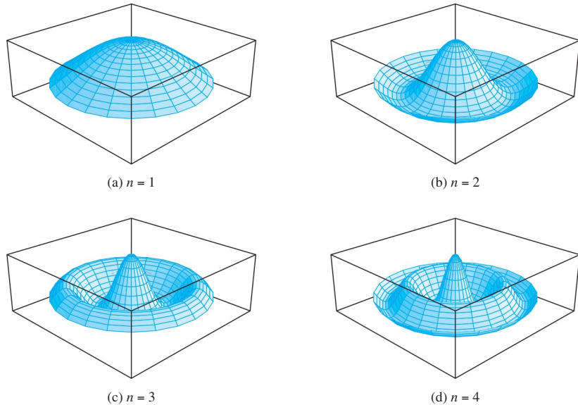
FIGURE 9.4.7. The surface u = J_0(\gamma_n r/c) for n = 1, 2, 3, 4 .
