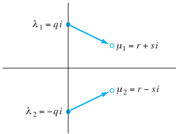
FIGURE 7.3.10. The effects of perturbation of pure imaginary roots.
