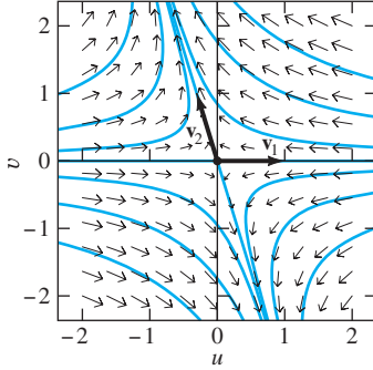
FIGURE 7.4.11. Phase plane portrait for the linear system in Eq. (22) corresponding to the critical point (7, 0) .
