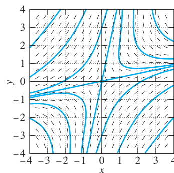
FIGURE 7.2.14. Saddle point (0, 0) .
