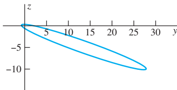
FIGURE 6.4.15. yz -projection of the orbit of Halley's comet.
