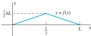
FIGURE 8.6.2. The initial position of the plucked string of Example 2.
