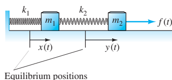
FIGURE 5.1.1. The mass-and-spring system of Example 1.
