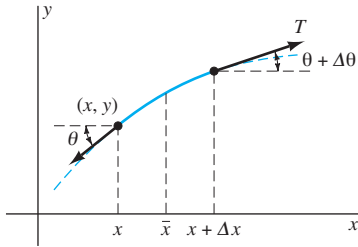
FIGURE 2.8.7. Forces on a short segment of the whirling string.
