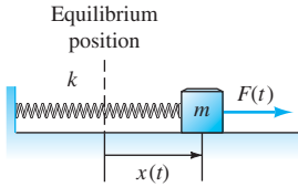
FIGURE 8.4.1. A mass-and-spring system with external force.
