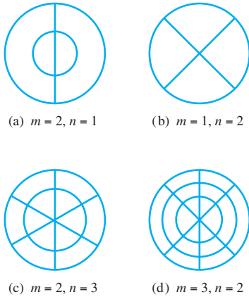
FIGURE 9.5.6. Typical nodal circles and radii for a vibrating circular membrane.
