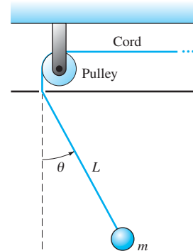
FIGURE 3.6.6. A variable-length pendulum.
