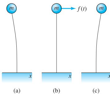
FIGURE 7.6.12. Equilibrium positions of a mass on a filament: (a) stable equilibrium with x < 0 ; (b) unstable equilibrium at x = 0 ; (c) stable equilibrium with x > 0 .
