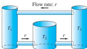
FIGURE 5.4.5. The three brine tanks of Example 4.
