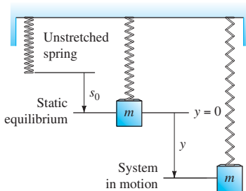
FIGURE 2.4.2. A mass suspended vertically from a spring.
