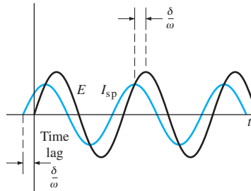
FIGURE 2.7.5. Time lag of current behind imposed voltage.
