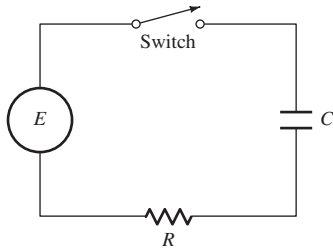
FIGURE 2.7.8. The circuit for Problems 7 through 10.
